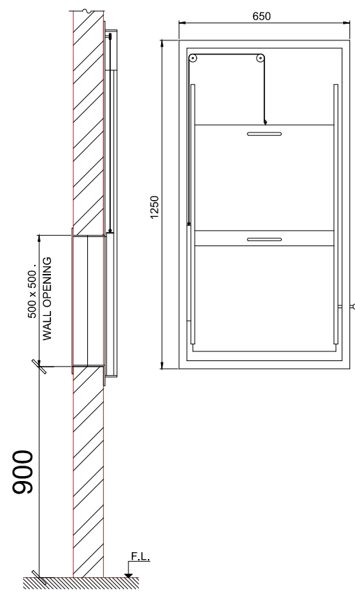
ENLARGED DETAIL OF SS VERTICAL SLIDING DOOR
